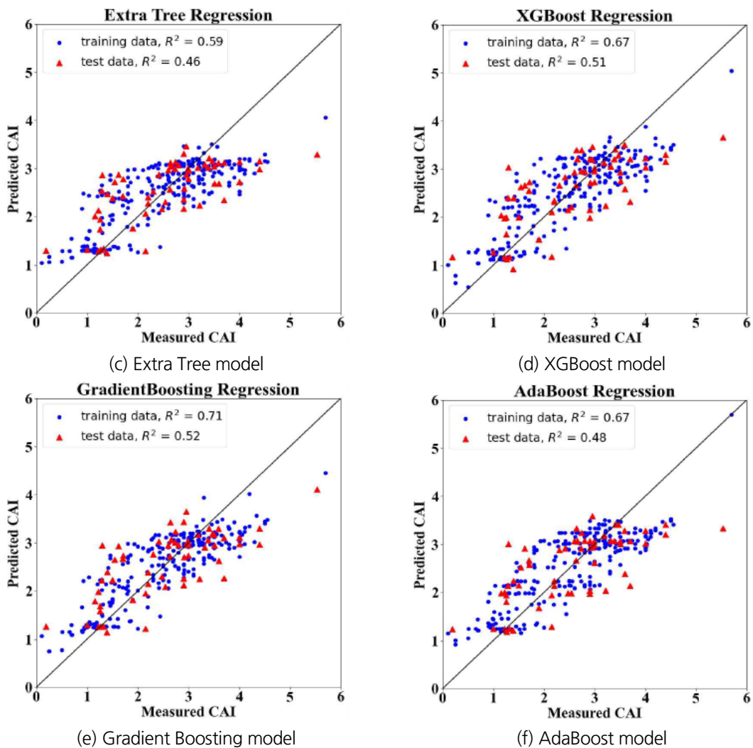
Fig. 6. Results of comparison between measured and predicted CAI for machine learning models in all rock types (continued)
